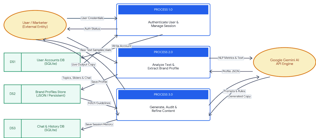
System Data Flow Diagram
